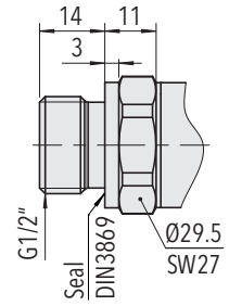
8292.XX.XX21.XX.XX.XX (≤ 600 bar)
