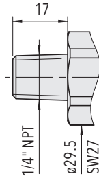
8292.XX.XX30.XX.XX.XX (≤ 1000 bar)
