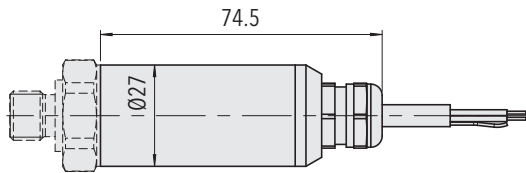
8292.XX.XXXX.78/80.XX.XX
